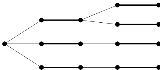
Figure 1: An M -alternating tree
