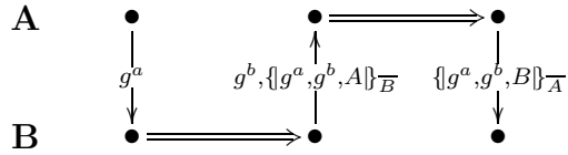
Fig. 1. ISO-9798-3 as arrows-and-messages
