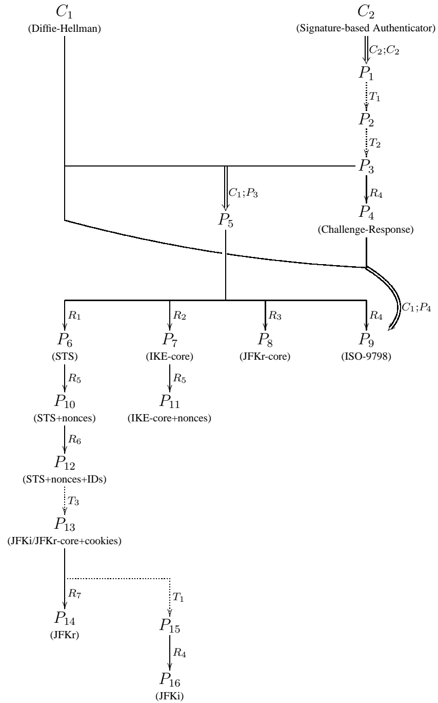
Fig. E.1. Derivation graph of the STS protocol family
