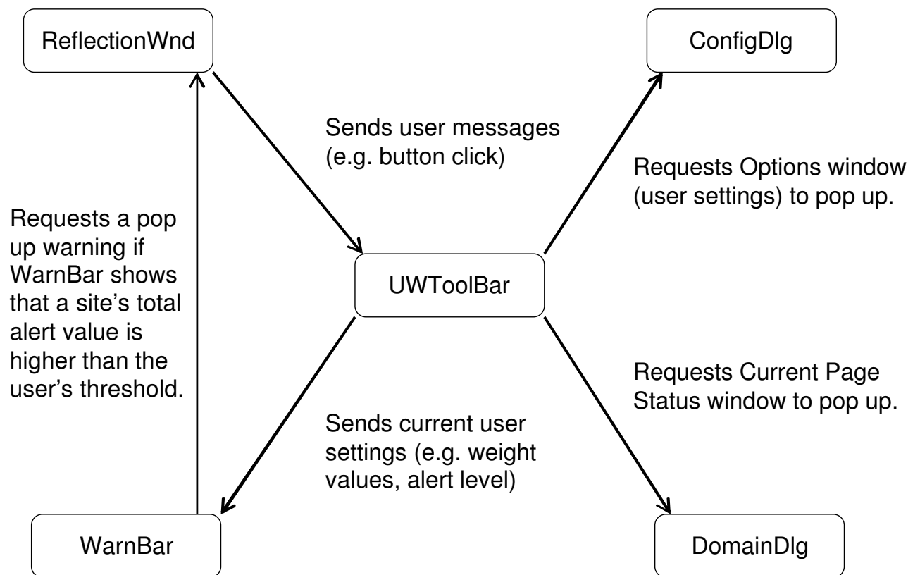
Figure 1. SpooferGuard architecture
