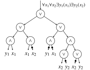
Fig. 1: Quantifier graph in NNF.
