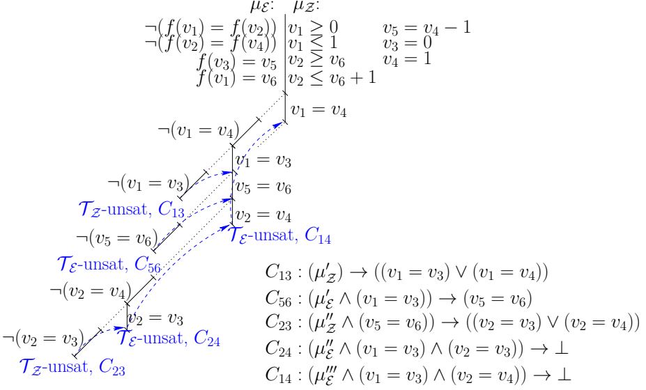
Figure 33.6. The DTC search tree for Example 33.6.3 on \mathcal{T}_Z \cup \mathcal{T}_\varepsilon , with no e_{ij} -deduction. v_1, \dots, v_6 are interface terms. \mu'_{\mathcal{T}_i}, \mu''_{\mathcal{T}_i}, \mu'''_{\mathcal{T}_i} denote appropriate subsets of \mu_{\mathcal{T}_i} , \mathcal{T}_i \in \{\mathcal{T}_\varepsilon, \mathcal{T}_Z\} .
