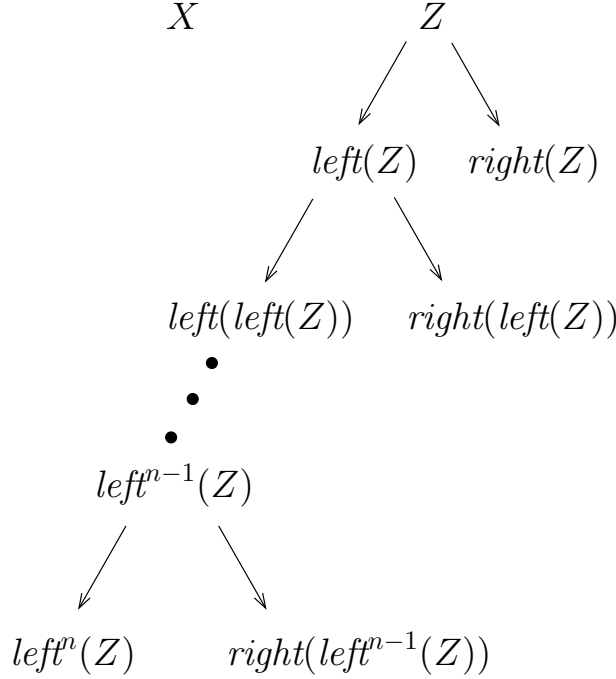
Figure 6. Term graph for Example 5.1
