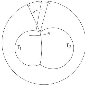
FIGURE 7.9. f backtracks at the points of intersection of the exterior components.
