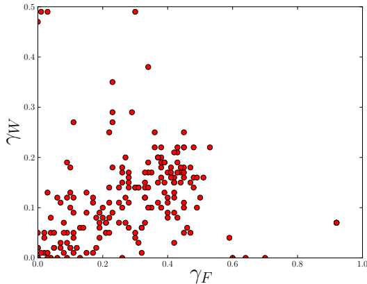
Figure 4: Scatter plot of \gamma_W versus \gamma_F .
