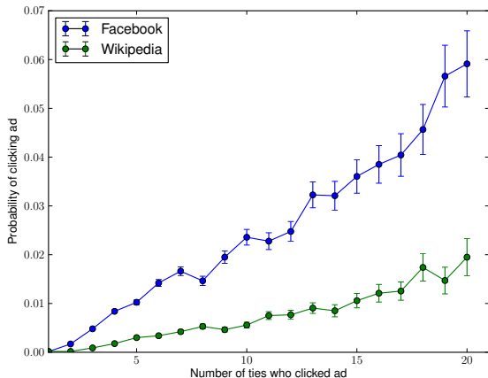
Figure 2: Probability of clicking on an ad given that k ties clicked on it.
