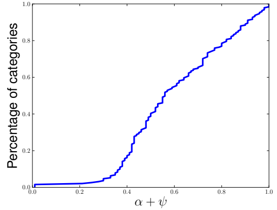
Figure 3: Cumulative distribution function of the value \alpha + \psi for all of the second-level categories.
