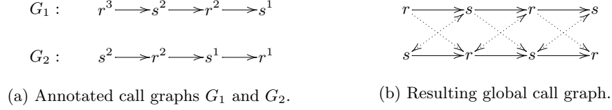
Fig. 7. Global call graph for two call graphs G_1 and G_2 .
