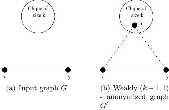
Figure 2: Illustrative example of the difference between weak and strong anonymity.
