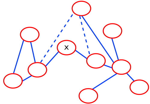
(b) (4,1) -anonymous transformation of G
