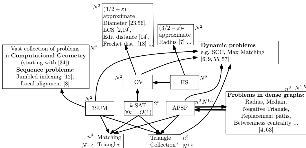
■ Figure 1 Partial summary of the implications of the main conjectures. An arrow from problem A to problem B , where A has a(n) next to it, B has b(n) next to it, implies that A \leq_{a,b} B . When the inputs are graphs, n stands for the number of nodes. N always stands for the total input size. When both n and N are present for a problem, we assume that N = n^2 ; the meaning is that the reductions are only for dense graphs in which case the input size is quadratic in n . For k -SAT, n denotes the number of variables. For the dynamic problems, different key problems can be reduced to different key problems, and the update/query time tradeoffs vary. References are not comprehensive.
